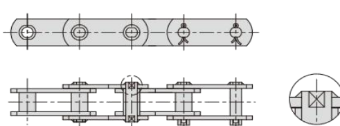
5. Welded pins with plates
