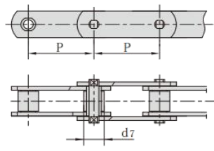
2. with S small rollers type
