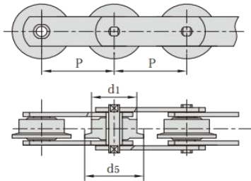
4. with F flanged rollers type
