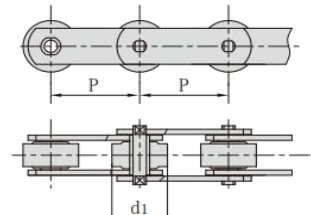
3. with P large rollers type
